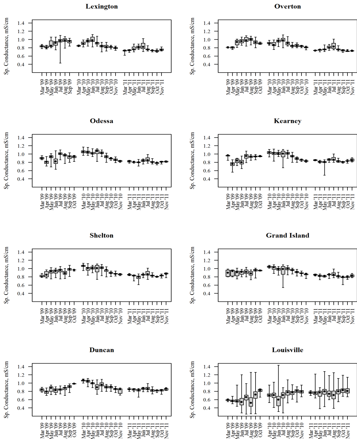
Figure B-14. Spatial Variation, Monthly Specific Conductance, Interquartile Ranges, Platte River, NE
