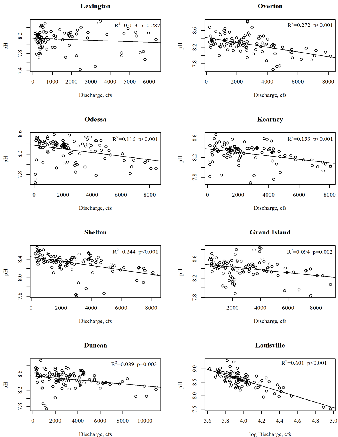
Figure B-21. Scatter Plot, pH, Platte River, NE
