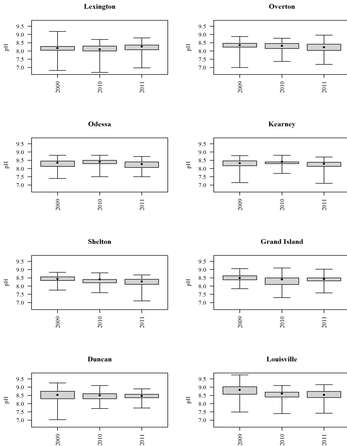
Figure B-9. Spatial Variation, Annual pH, Interquartile Ranges, Platte River, NE
