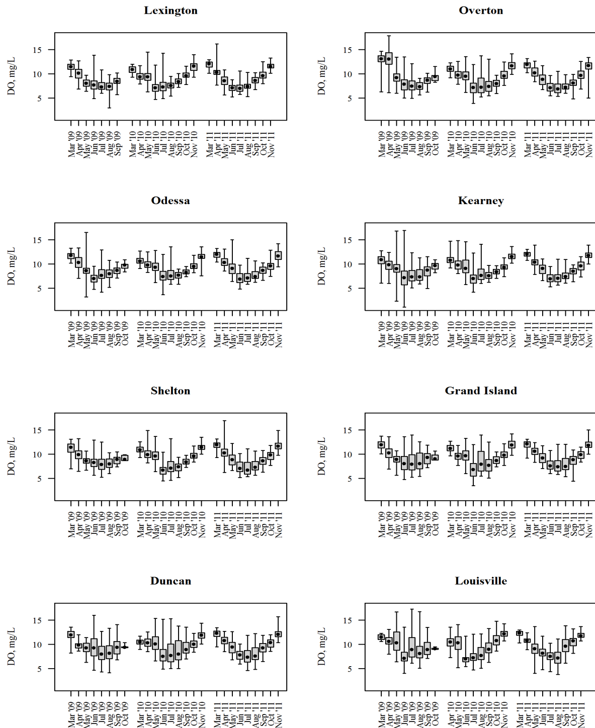
Figure B-17. Spatial Variation, Monthly Dissolved Oxygen, Interquartile Ranges, Platte River, NE
