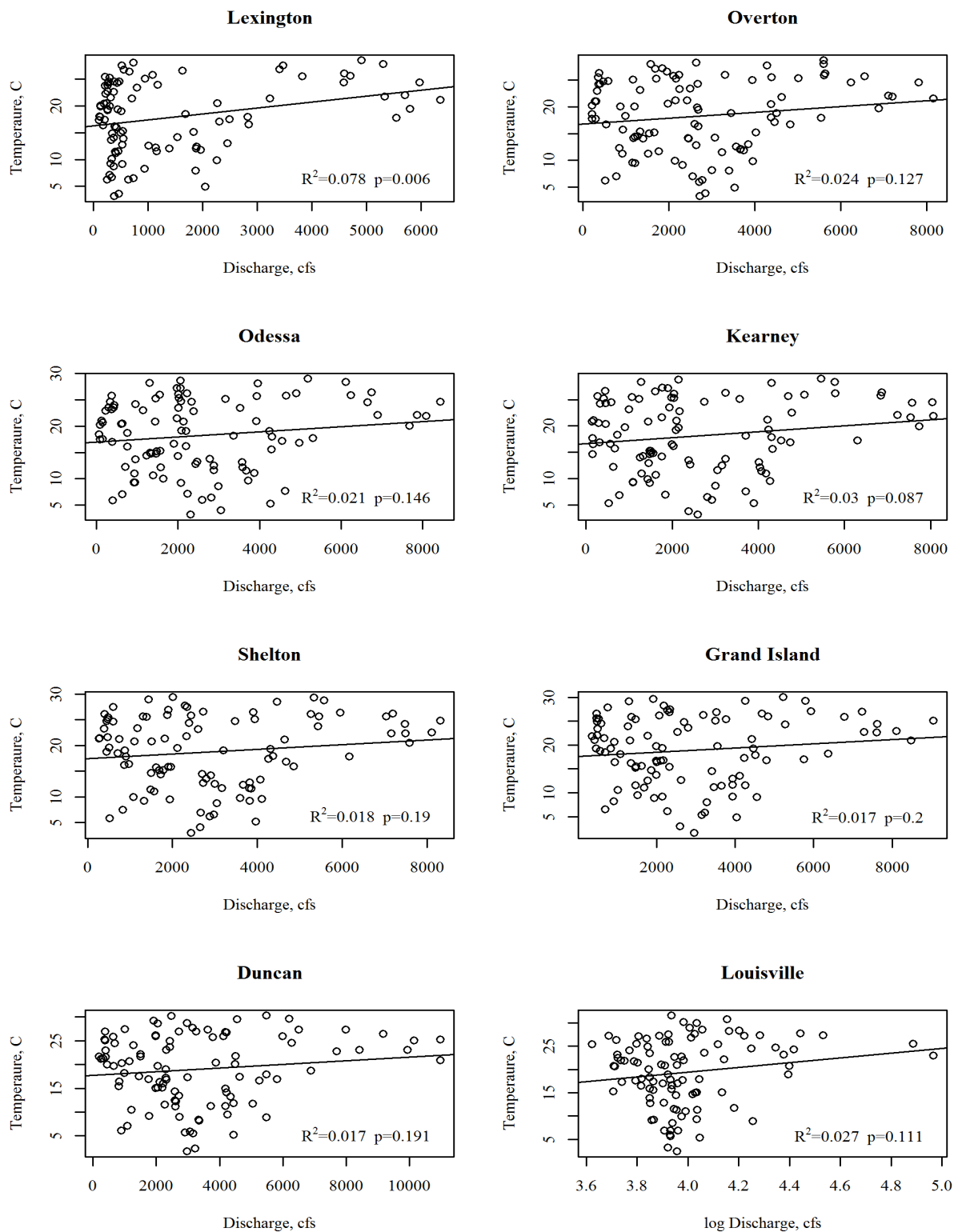
Figure B-19. Scatter Plot, Temperature, Platte River, NE
