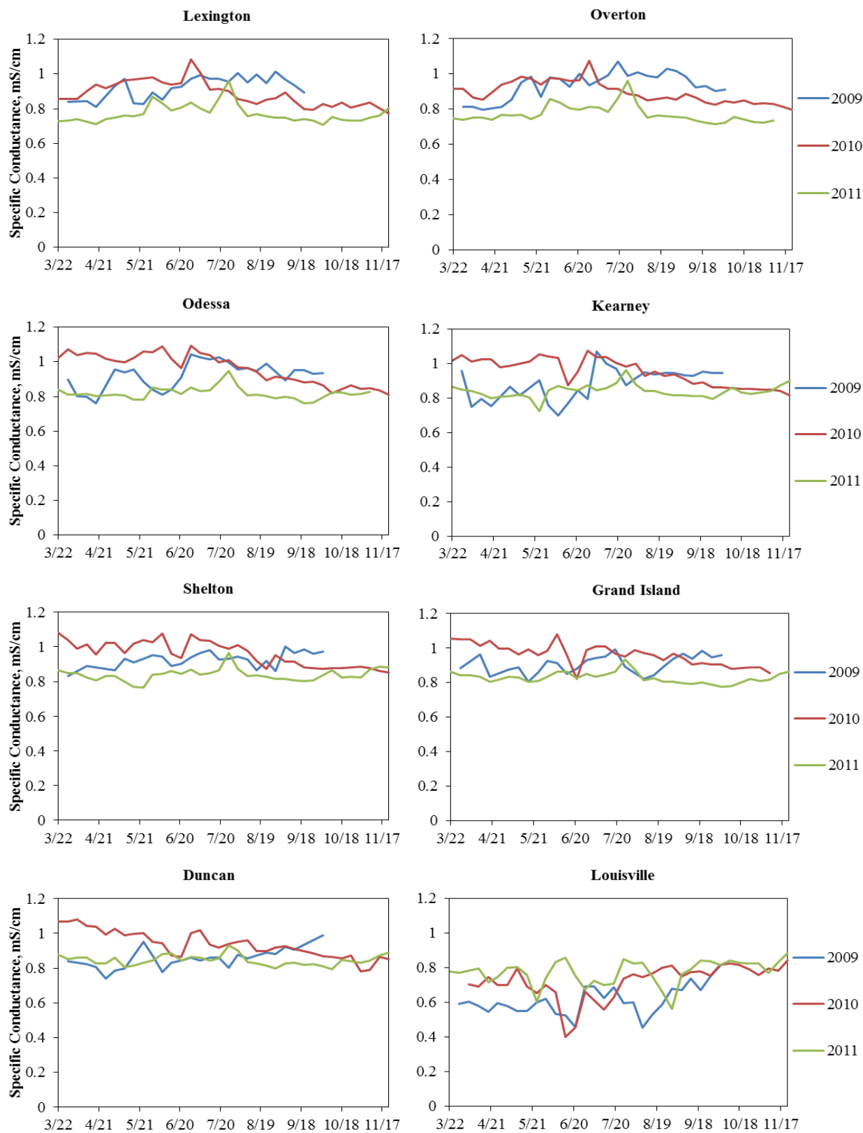
Figure B-2. Temporal Variation, Specific Conductance, Weekly Mean, Platte River, NE
