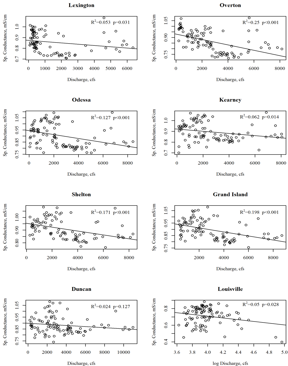
Figure B-20. Scatter Plot, Specific Conductance, Platte River, NE
