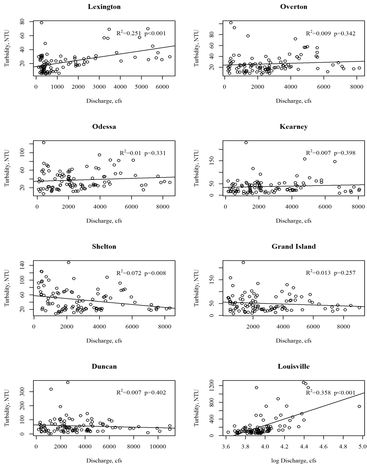
Figure B-22. Scatter Plot, Turbidity, Platter River, NE
