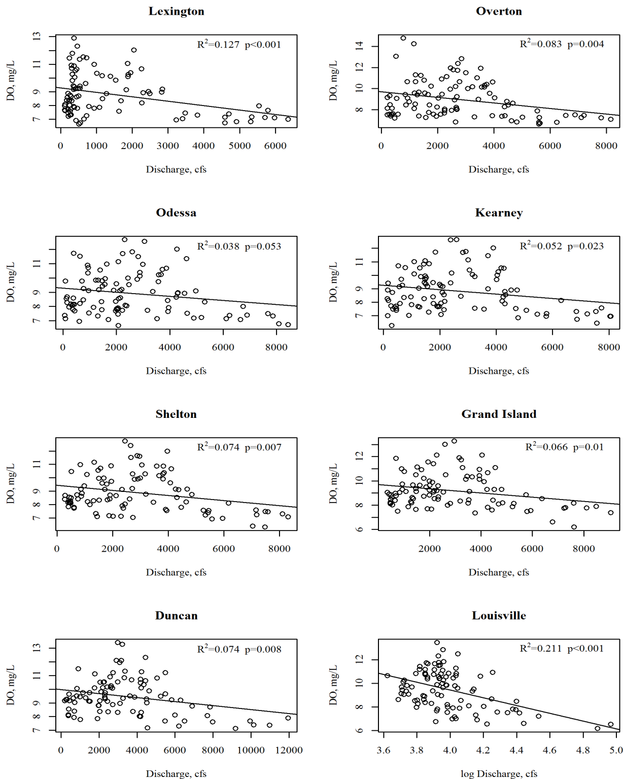
Figure B-23. Scatter Plot, Dissolved Oxygen, Platte River, NE
