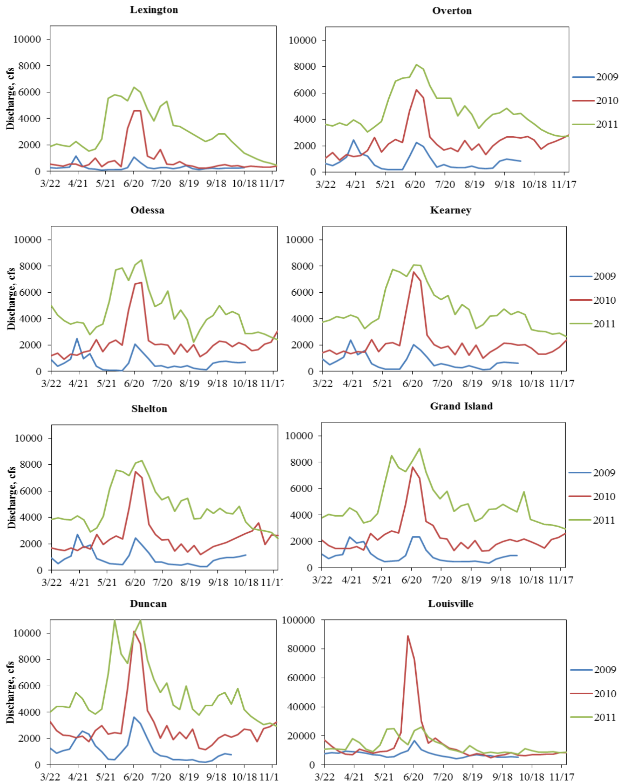
Figure B-6. Temporal Variation, Discharge, Weekly Mean, Platte River, NE
