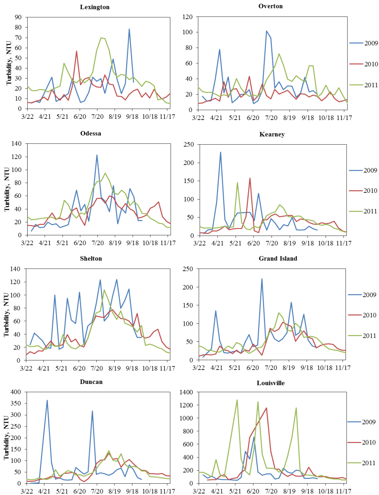
Figure B-4. Temporal Variation, Turbidity, Weekly Mean, Platte River, NE
