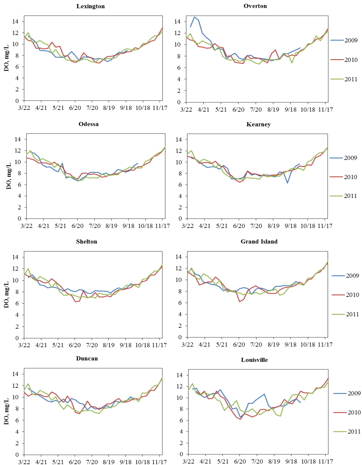
Figure B-5. Temporal Variation, Dissolved Oxygen, Weekly Mean, Platte River, NE
